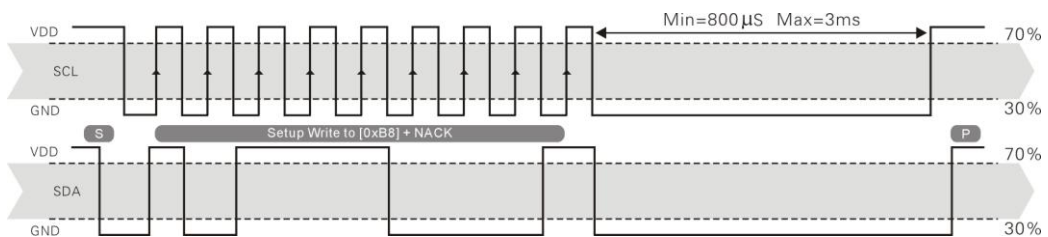
Figure 14: Wake-up sensor
